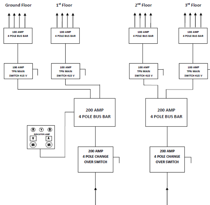
3 Phase 4 Wire 415 Volt Incoming Line From CESC Meter Room
